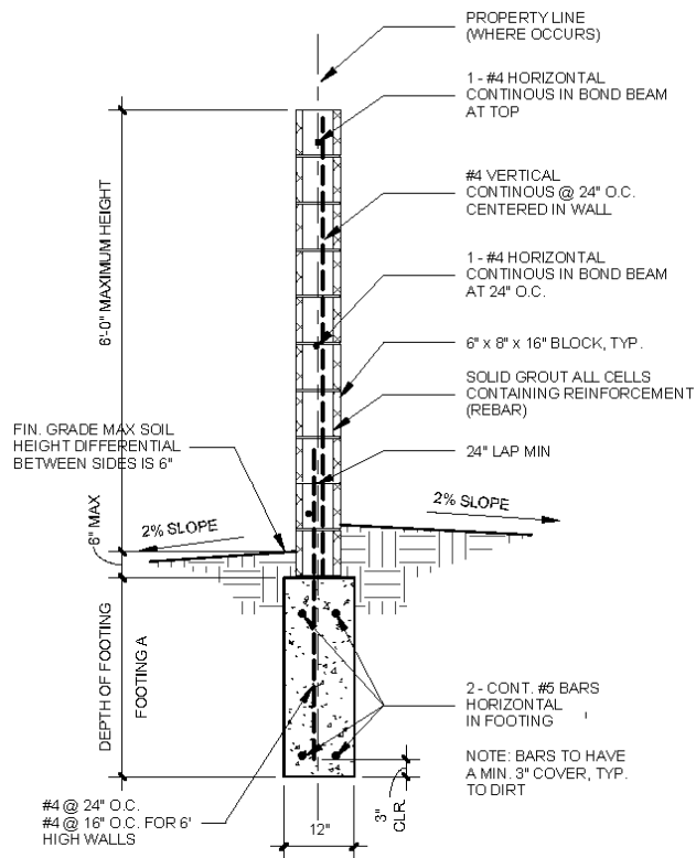
BLOCK WALL SECTION A 1/2" = 1'-0"
