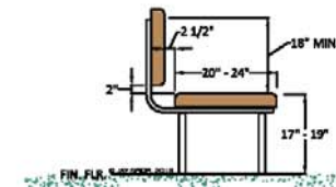
BENCH SIZE, SUPPORT & CLEAR FLOOR SPACE 11B-903
