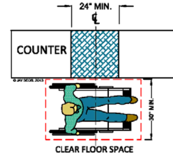
ALTERATION OF SALES AND SERVICE COUNTERS 11B-904.4 (EXCEPTION)
